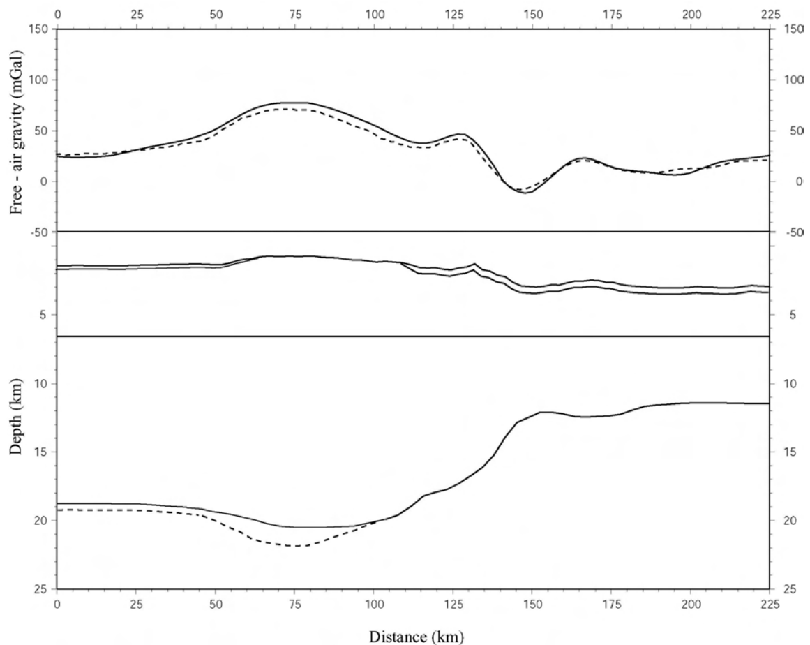
Figure 30. Gravity modeling solution along reference transect 2 (corrected Moho geometry). The solid line represents the observed gravity anomaly field, whereas the dashed line corresponds to the calculated gravity anomaly field. The dashed line in the crustal model (bottom panel) shows the extent to which the crustal root beneath the crest of the ridge was modified.
